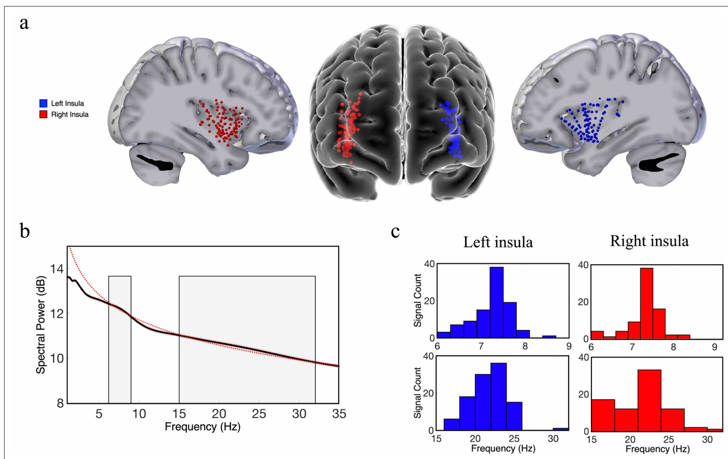
Figure 1. Theta-band and beta-band frequency oscillations in the human insula. (a) Lateral and frontal views of the brain showing electrodes in the left insula ( n=125 ) and right insula ( n=114 ) across all participants. (b) An oscillation-detection algorithm known as multiple oscillations detection algorithm (MODAL) detected theta ( \sim 6 – 9 Hz) and beta ( \sim 15 – 32 Hz) oscillations across all electrodes in the insula (Materials and methods). The black line depicts the power spectrum, the red dotted line depicts the 1/f regression line, and the red shaded region around the spectrum represents the standard error of the mean power for each frequency. Gray shaded regions indicate the detected frequency bands at which the power spectrum was higher than the 1/f background signal. (c) The distribution of the peak frequencies detected across all insula electrodes. In the left insula, 90% of electrodes had theta oscillations and 99% had beta oscillations. In the right insula, 80% of electrodes had theta oscillations and 81% had beta oscillations. Peak frequencies of theta and beta oscillations appear to have relatively normal distributions across the insula.
